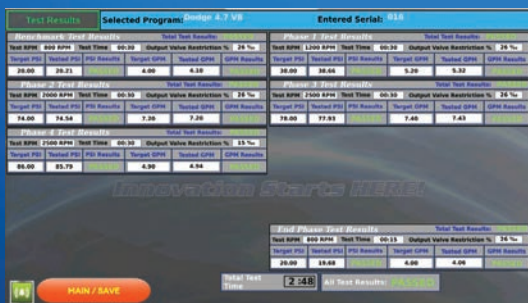
Pump Test Result
